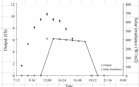
Fig. 2. Battery-Based System with 75W PV Panel
